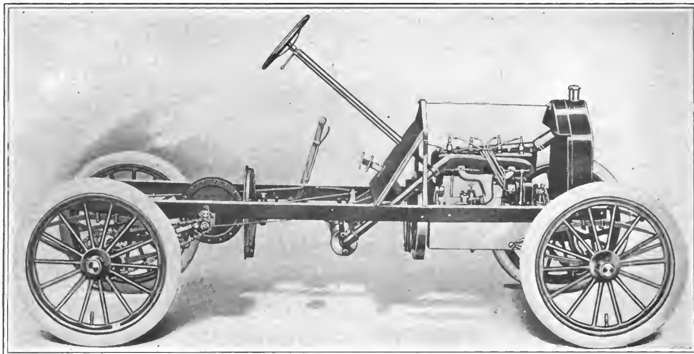
Fig. 1—The chassis of the 1912 Metz car is shown here in elevation
